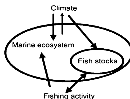
Fig. 41. Schematic representation of the impacts of climate change and fishing activity on the marine ecosystem and its fish component (Source: http://www.pnas.org/content/104/50/19709.full )
